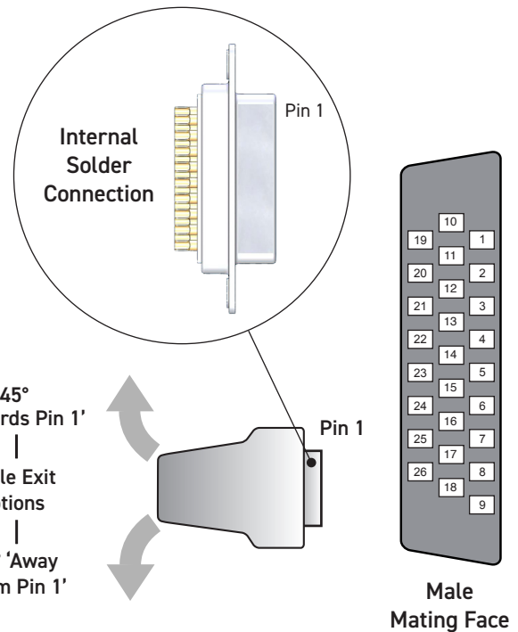
26-Pin D-Type Cable Connector with Backshell
