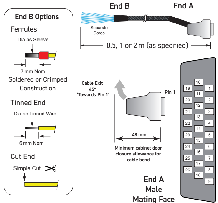
26-Pin D-Type Unterminated Cable Assembly
