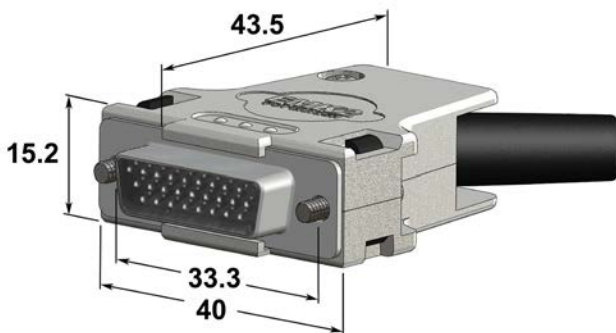
Connector Dimensions
