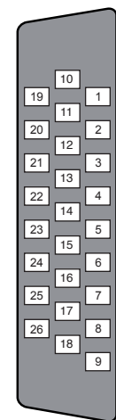
Male Mating Face
