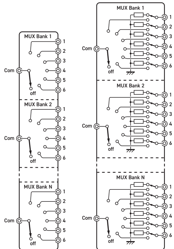
60-800 Unterminated Microwave MUX - up to 16 Multiplexers can be supported
