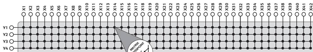
40-505-001 42x4 Matrix Switching Diagram
